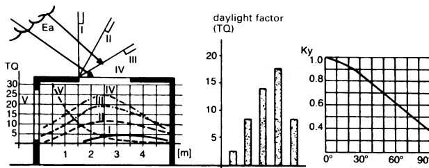
(a) Comparative variations in the daylight factor for side and overhead illumination with various inclinations of the rooflights (b) Diminution factor K_y as a function of the inclination \gamma of the glazing in shed roofs
